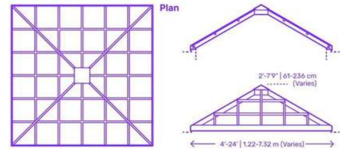
Skylight - Pyramid, 30 Degree
